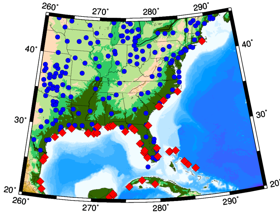
GPS stations (blue) and locations of hurricane landfalls
